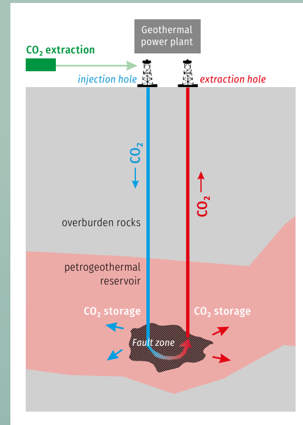
EGS-CO 2 installation
